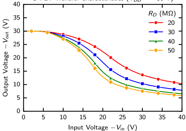
O-FET Transfer Characteristics ( V_{DD} = -30\text{ V} )
